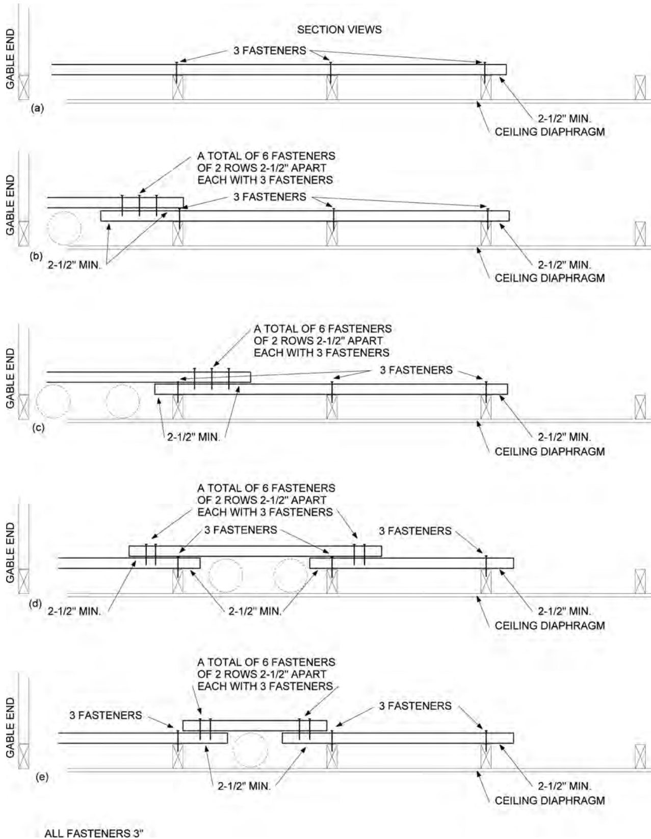
[BS] FIGURE C104.2.8(1) SPliced HORIZONTAL BRACES
