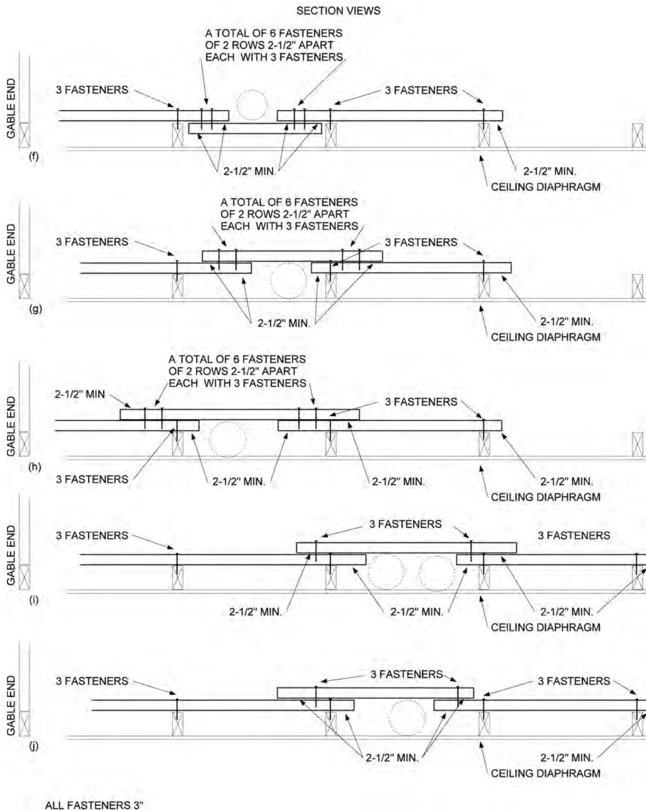
[BS] FIGURE C104.2.8(2) SPliced HORIZONTAL BRACES
